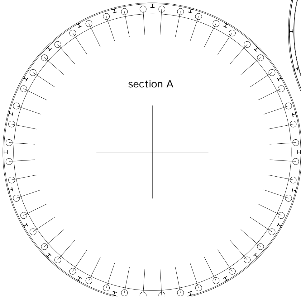
Titan II Interstage Cross-Section 1/24th scale
